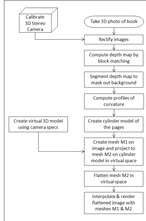
Figure 3. Method pipeline
